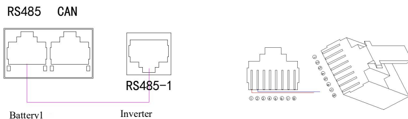
Figure 7 communication cable connection between battery pack and inverter
