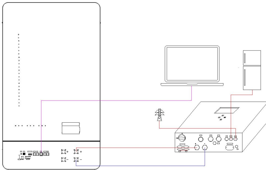
Figure 4 single battery connect with inverter
