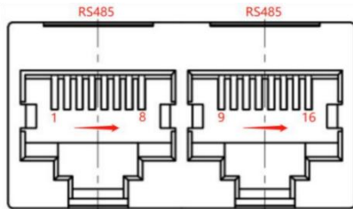
parallel communication
